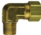
(1) 69749 3/8" NPT To 5/8" Tube 90*
